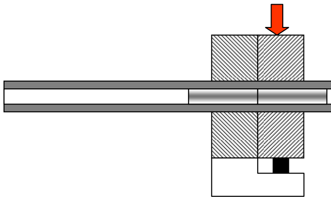
Figure 7: Basic principle of the tube cutting process.
