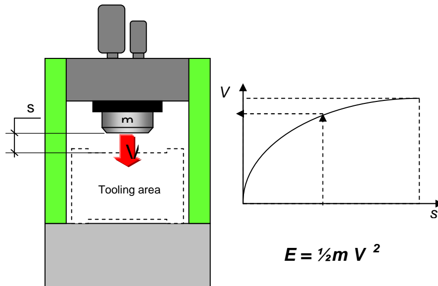
Figure 8: Principle of ADIPRESS' machines and control of the energy.
