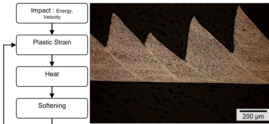
Figure 1: Principle of development of adiabatic shear bands and micrograph of an example of adiabatic shear band produced by High Velocity Machining [1].
