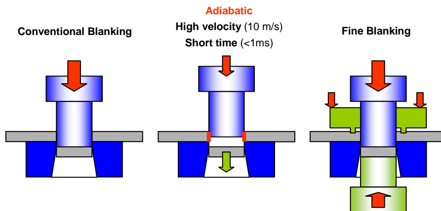
Figure 2: Adiabatic blanking principle.
