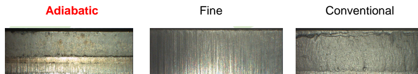
Figure 3: Blanked surfaces of steel part (4 mm thick): adiabatic, fine and conventional blanking [2].
