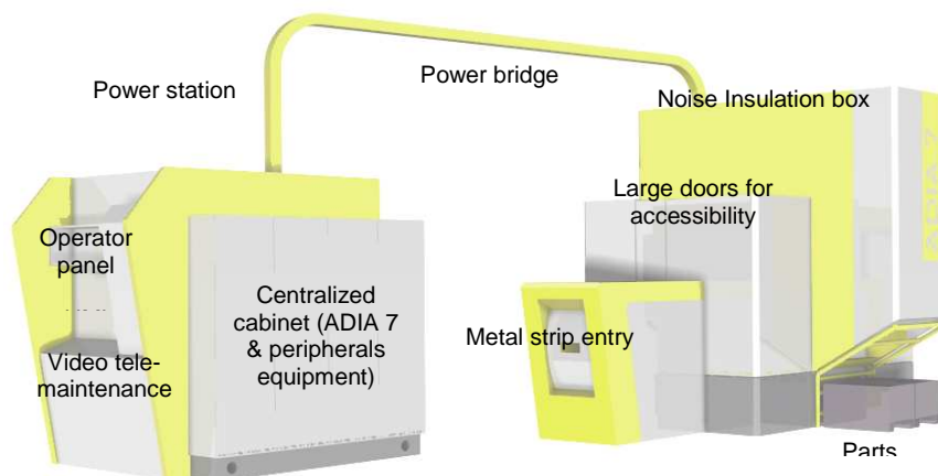
Figure 9: General presentation of ADIA 7.
